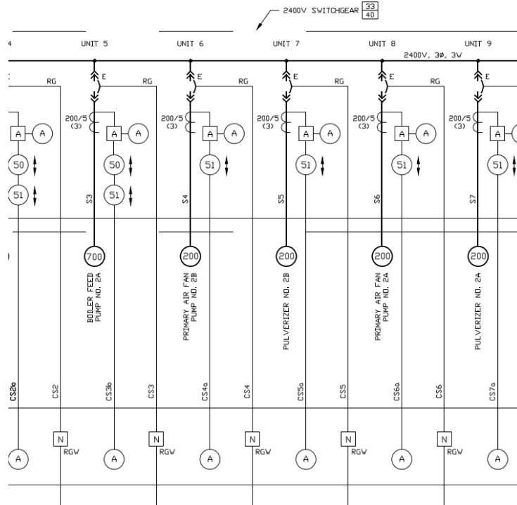
Figure 2: One Line Diagram
